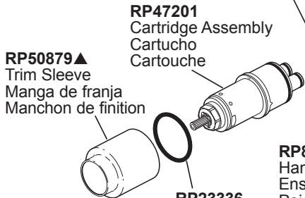
RP23336 O-Ring Anillo "O" Joint torique
